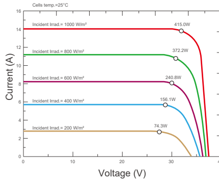
Current-Voltage & Power-Voltage Curves (RMHB54-415AB3)
