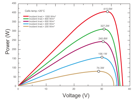
Current-Voltage & Power-Voltage Curves (RMHB54-415AB3)
